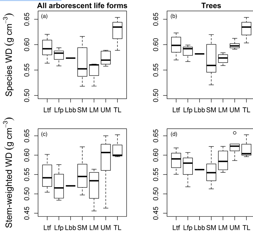
FIGURE 6 Plot-level wood density variation across forest types including: Lowland (Ltf = Lowland terra firme, Lfp = Lowland floodplain, Lbb = Lowland bamboo dominated forest; <500 m), submontane (SM: 500–1500 m), lower montane (LM: 1500–2500 m), upper montane (UP: 2500–3400 m) and tree line (TL: >3400 m) for (a) species mean WD including all arborescent life forms and (b) tree species. (c) Stem-weighted WD for all arborescent life forms and (d) tree stems. Box plots show 25% quartile, median and 75% quartile of the distribution (horizontal lines). Forest types are defined based on Young (1992) and Pennington et al. (2004).
