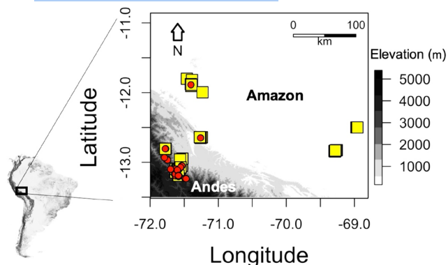
FIGURE 1 Location of the 51 wood collection sites (red circles) and the 41 permanent forest plots (yellow squares) on the eastern slope of the Peruvian Andes along an elevational gradient extending from the tree line at 3700m to the Amazon basin at 190m.
